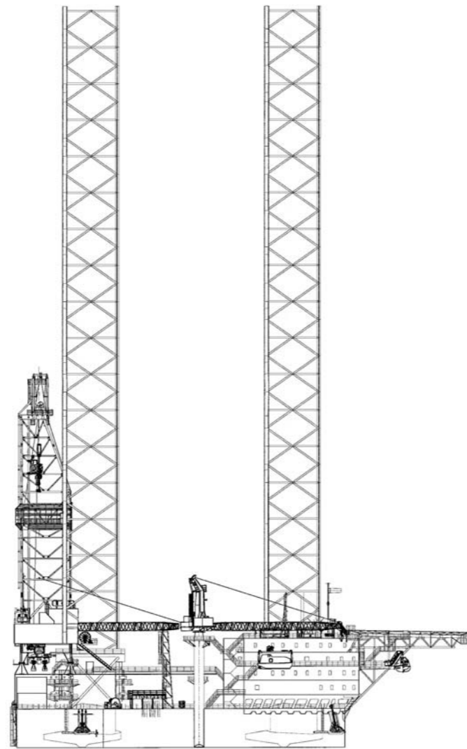
GENERAL ARRANGEMENT OUTBOARD PROFILE
