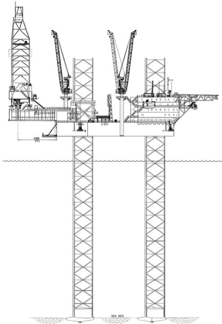
GENERAL ARRANGEMENT PROFILE (CANTILEVER FULLY RETRACT)
